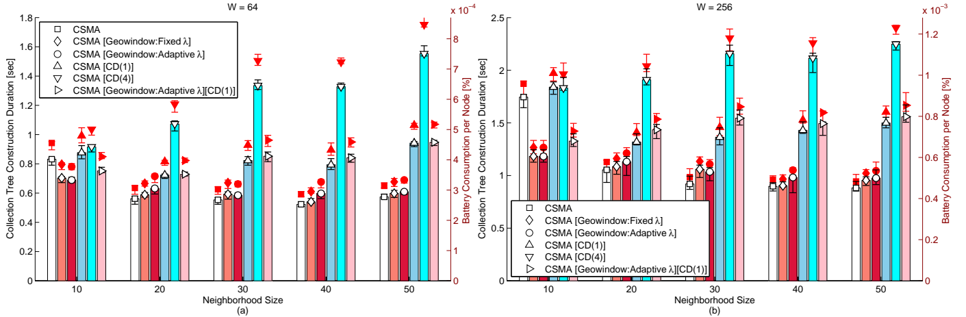
Figure 14: Influence of the MAC mechanisms on CTC duration and energy consumption. The bars are corresponding to the left axis, which indicates duration. The markers above the bars indicate energy consumption, which is corresponding to the right axis. Utilizing cost retransmission causes significant increase in duration and energy consumption, which reduces the efficiency of the CSMA [CD(x)] mechanisms for periodical execution during the data gathering phase. The Geowindow-based mechanisms demonstrate short duration and low energy consumption, because they do not alter the original contention window size, and they reduce the number of cost broadcasts.
