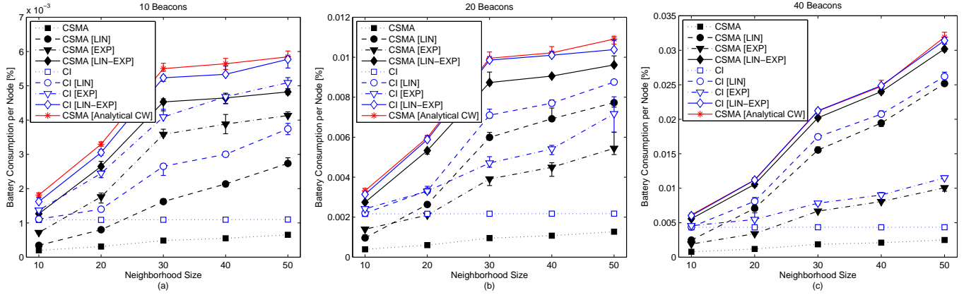
Figure 8: Influence of the MAC mechanisms and number of beacons on the average percentage of battery consumption per node.
