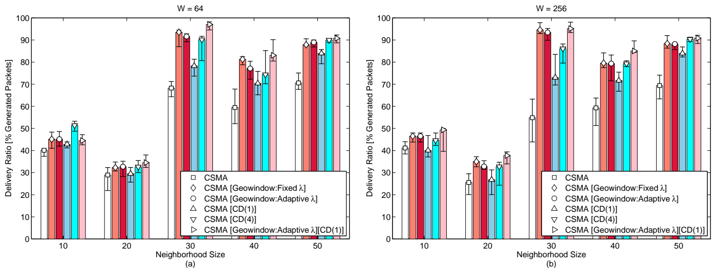
Figure 15: Percentage of packet delivery at the sink node. Through comparison with Figure 13, it can be observed that packet delivery performance depends on CTC accuracy. Here, CSMA:Geowindow [Adaptive \lambda ] shows up to 70% improvement over the CSMA mechanism.
