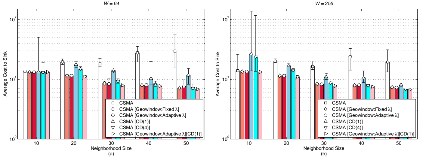
Figure 13: Influence of the MAC mechanisms on CTC accuracy defined as the average cost of the nodes towards the sink. CSMA has the lowest performance and presents significant variations which are due to the effects of collisions. Although employing cost retransmission through collision detection can improve CTC accuracy, this approach significantly increases CTC duration and energy consumption, as shown in Figure 14. The Geowindow-based mechanisms considerably improve CTC accuracy (up to 74%) without presenting long duration or high energy consumption (as Figure 14 shows).
