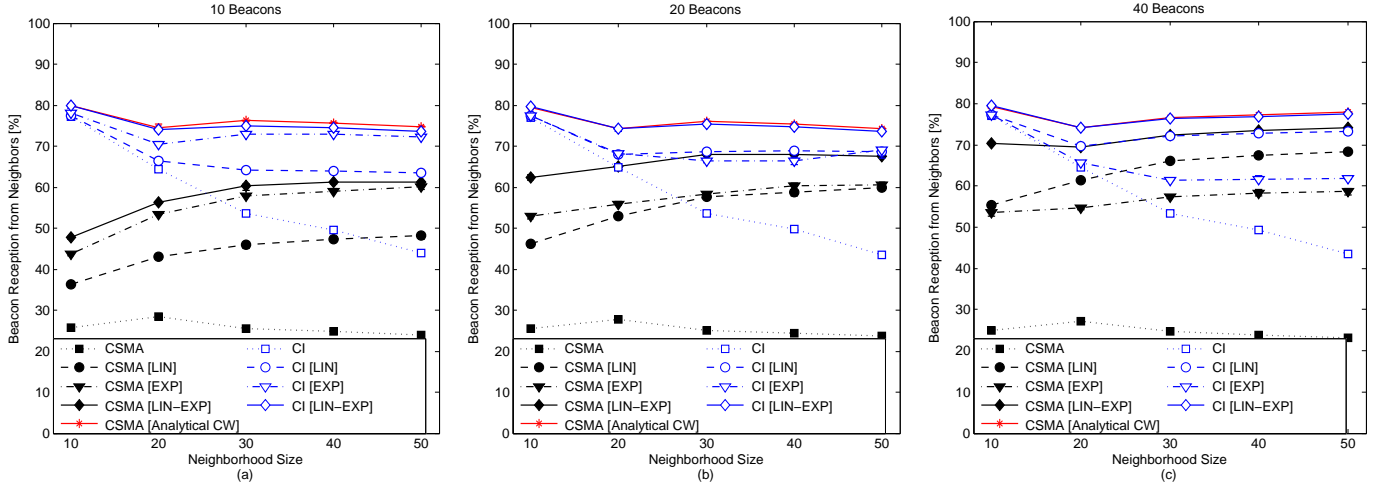
Figure 4: The average packet reception percentage of the nodes from those neighbors that their average link quality is higher than 10%. At low network densities the CI-based mechanisms present similar performance because the inter-beacon interval can effectively avoid collisions. However, as the neighborhood size increases, the performance of these mechanisms depends on the utilized backoff scheme. This figure also shows that the performance of the linear backoff scheme depends on network density and number of exchanged beacons. Also, the potential benefits of the mixed linear and exponential schemes can be observed.
