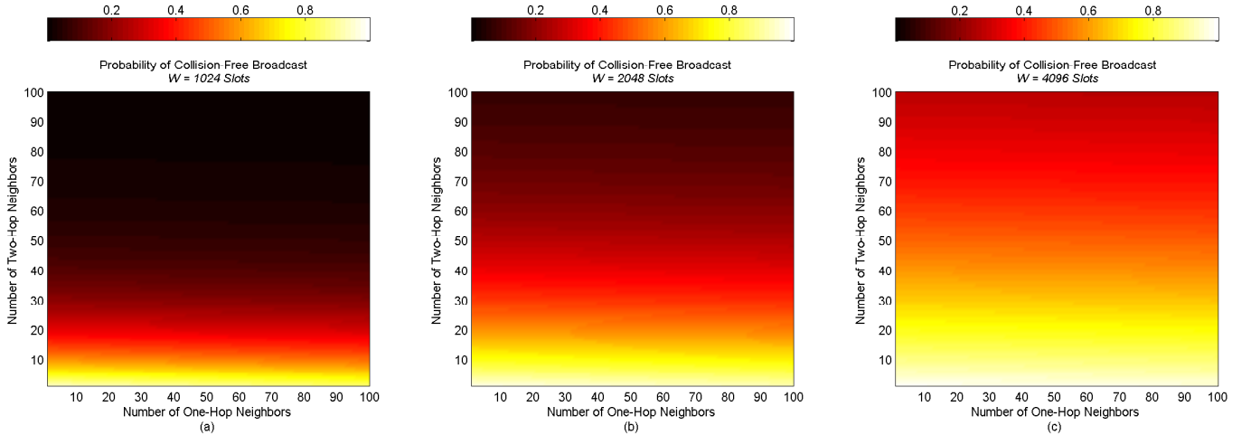
Figure 2: Mathematical analysis of collision-free broadcasting. Each sub-figure shows how changing the number of one-hop and two-hop neighbors affect the probability of collision-free broadcasting with a given contention window size. Since the carrier sensing mechanism of CSMA can significantly avoid one-hop collisions, this figure shows that broadcasting success probability mainly depends on the number of two-hop neighbors. Therefore, as most of the collisions are due to the hidden-node problem, the capture effect can be used for collision detection and packet recovery.
