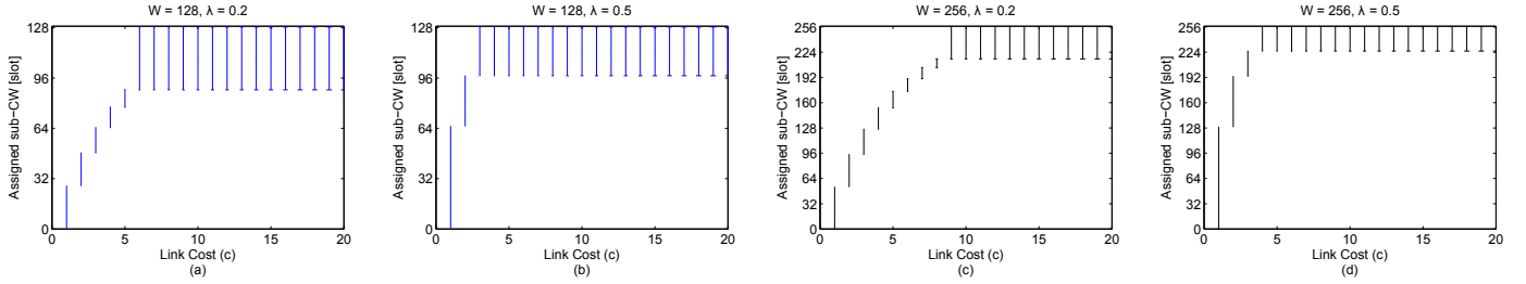
Figure 12: The assigned sub-CW corresponding to various cost values. Each vertical bar determines the length and position of the assigned sub-CW. The minimum assignable sub-CW size ( W_{th} ) is 8 slots. The Geowindow algorithm does not resize the original contention window duration; instead, it performs collision avoidance through sub-CW assignment and prioritization.
