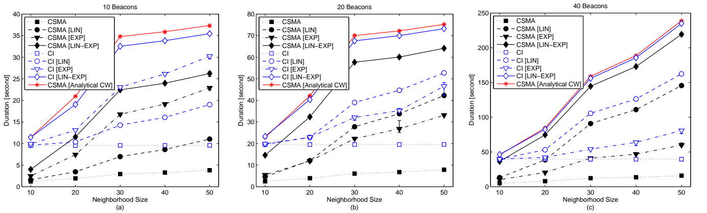
Figure 7: Influence of the MAC mechanisms and number of beacons on NDLE duration.
