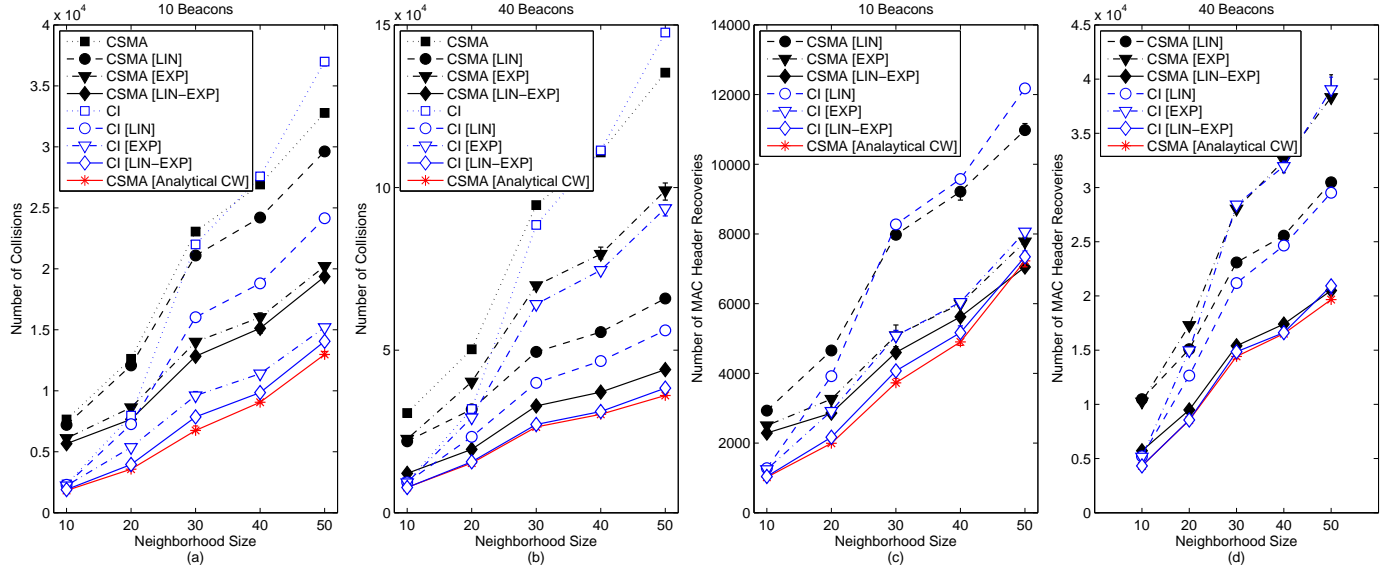
Figure 5: (a) and (b): The number of collisions that caused packet corruption. (c) and (d): The number of MAC headers that have been recovered during the collisions. Each collision corresponds to a packet arrival that causes the packet currently being received by the radio to be lost. Delivering partially recovered packets to the NDLE module allows for higher link estimation accuracy and more number of detected neighbors. Comparing the number of collisions and number of MAC header recoveries shows that increasing the number of collisions does not necessarily indicate higher number of MAC header recoveries. Specifically, for a given network configuration, increasing the number of collisions beyond a threshold value reduces the number of recoveries.
