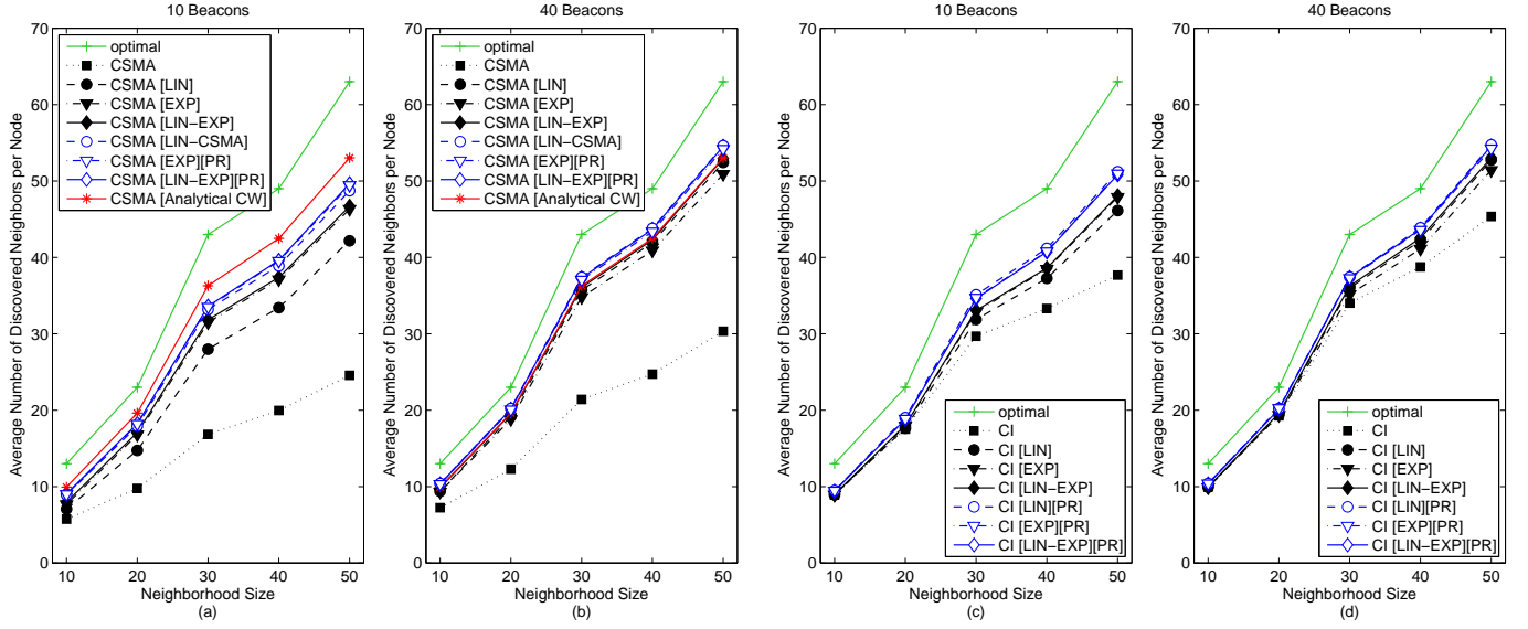
Figure 6: Influence of the MAC mechanisms and number of beacons on neighbor discovery. Increasing the number of beacon transmissions improves the number of discovered neighbors, because: (i) the probability of beacon receptions from the neighbors increases, and (ii) link variations can better be reflected.
