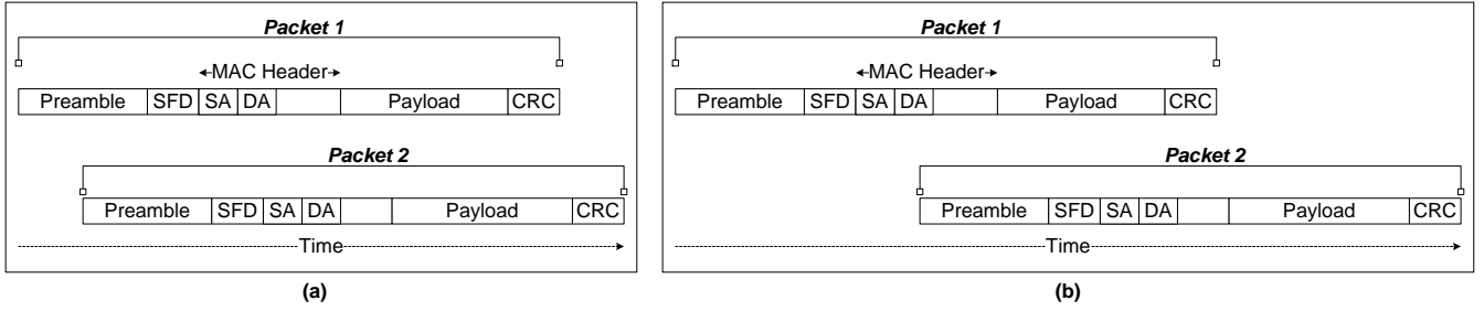
Figure 1: Collision detection through the capture effect. (a) This collision cannot be detected because it happens before receiving the SFD bytes. (b) This collision can be detected because it happens after receiving the SFD bytes.
