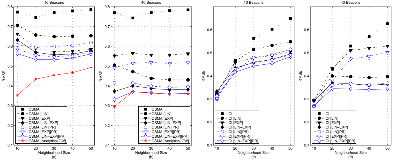
Figure 3: Influence of the MAC mechanisms and number of beacons on link estimation accuracy. The [LIN-EXP]-based schemes provide highest performance as they benefit from the fast contention window adjustment of the exponential scheme and lower variations of the linear scheme. For those mechanisms that utilize a contention window adjustment scheme, increasing the number of beacons allows for better contention window adjustment and higher accuracy. Increasing the number of beacons also contributes to accuracy improvement as it increases the granularity of link estimation.
