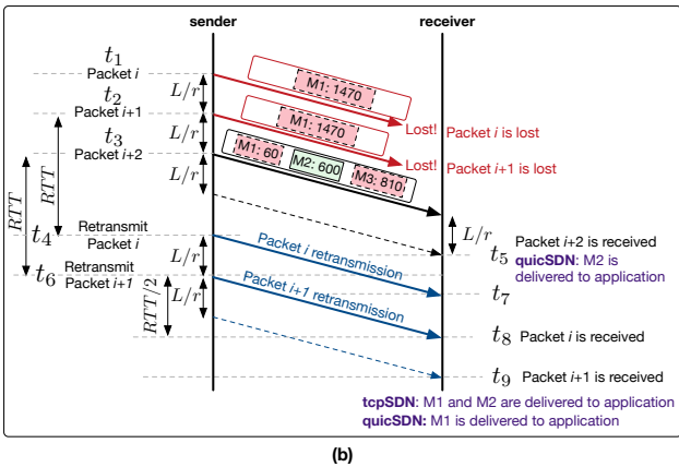
Fig. 11: The effect of packet loss and message size on the message delivery delay of tcpSDN and quicSDN. Here, L is the packet length (bits) and r is the transmission rate (bps) between the client and server. Red boxes show partial message inclusion in a packet and green boxes show complete inclusion of a message in a packet.
