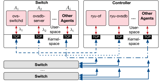
(a) tcpSDN Architecture.
